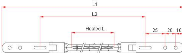
Metal Clip Type
